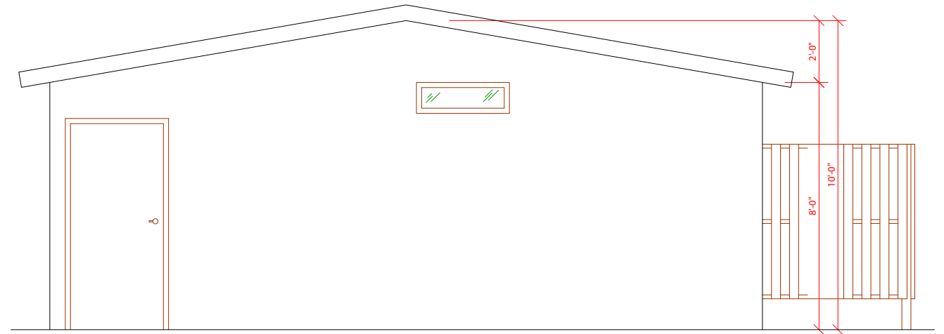
LEFT ELEVATION
