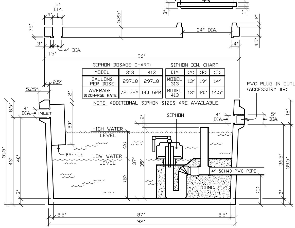
SECTION (TANK BASE, TOP, & COVER)
