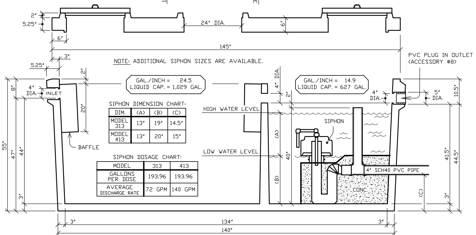
SECTION (TANK BASE, TOP, & COVER)
